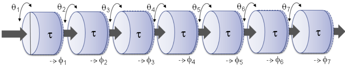
Figure 28 Model of concatenated birefringent sections each with retardation \tau , axis angle \theta and output phase \phi
