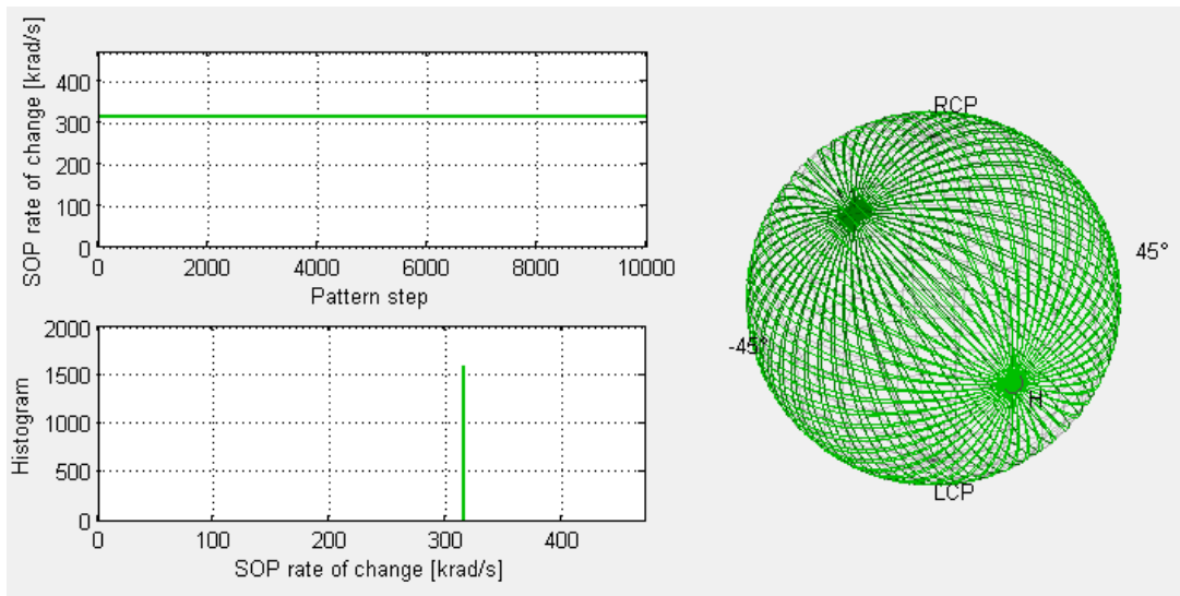
Figure 37 Illustration of Spinning Coin pattern mode
