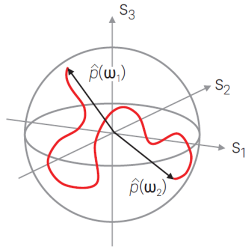
PSP spectrum
