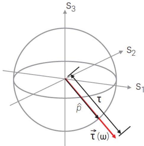
PMD vector in Stokes space
