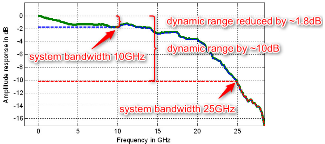
Figure 48 Flattened frequency response using de-emphasis
