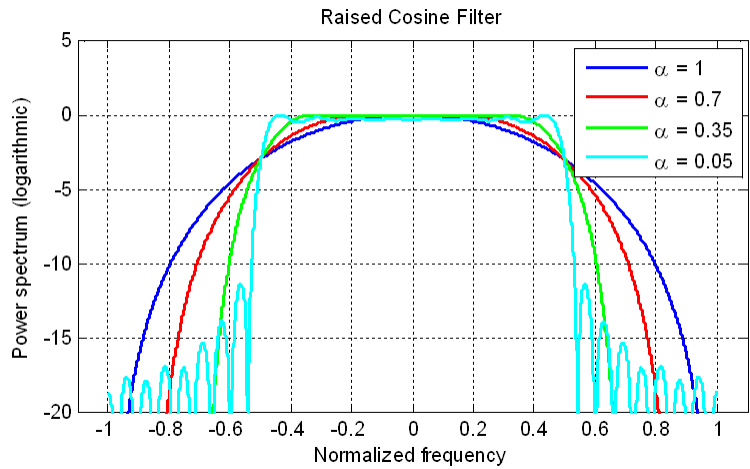
Figure 25 Spectrum (log) of a pulse shaping filter using a raised-cosine filter with different roll-off factors
