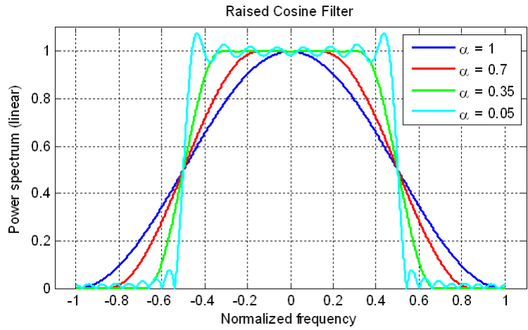
Figure 24 Spectrum of a pulse shaping filter using a raised-cosine filter with different roll-off factors
