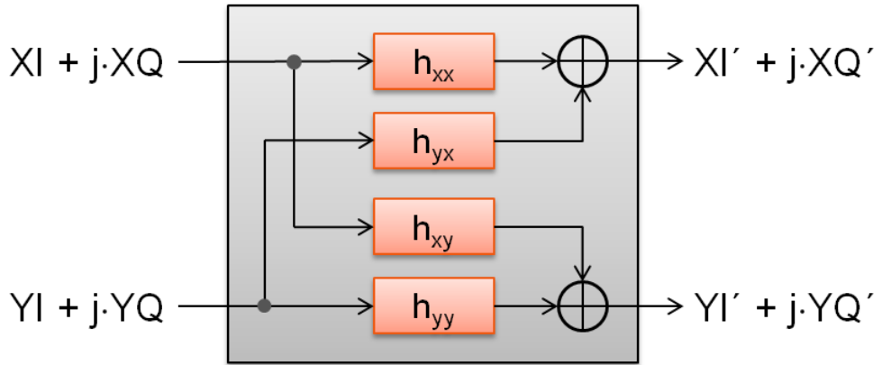
Figure 27 PMD Filter Structure
