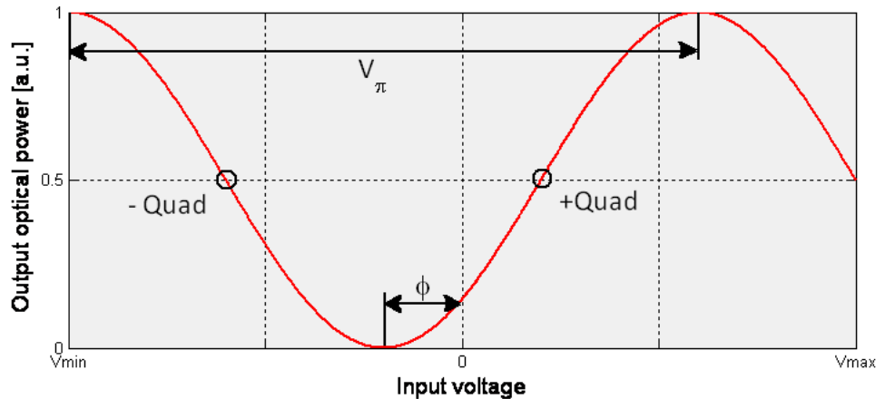
Figure 44 E/O modulator transfer function
