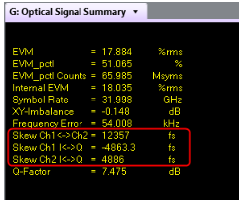
Figure 50 Skew measurement results in VSA
