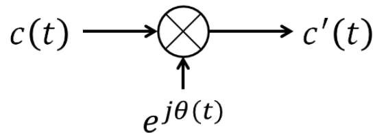
Figure 32 Illustration of adding phase noise to a complex signal
