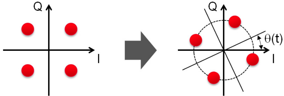
Figure 33 Illustration of the effect of phase noise / IQ rotation on the constellation diagram
