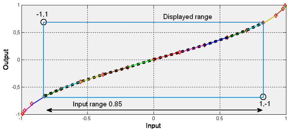
Figure 45 Non-linear transfer function using an arcsine as example
