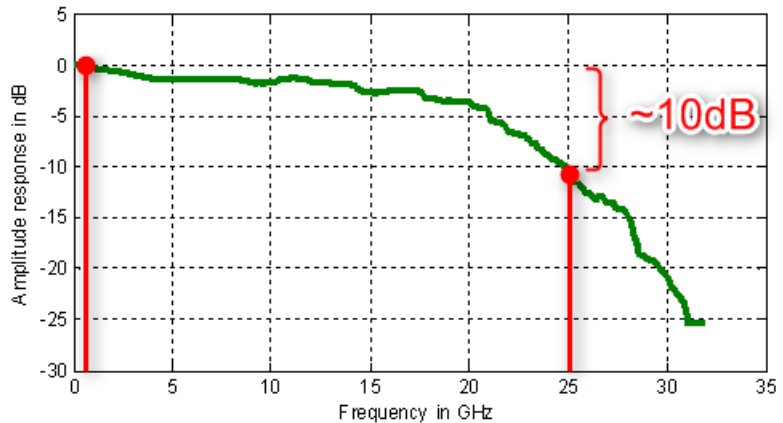
Figure 47 Exemplary frequency response
