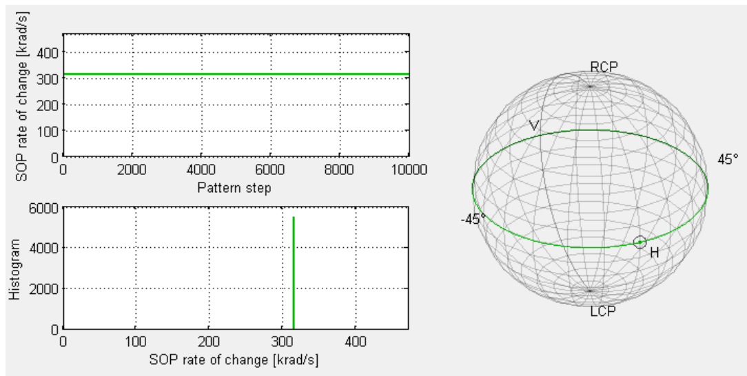
Figure 36 Illustration of Great Circle pattern mode
